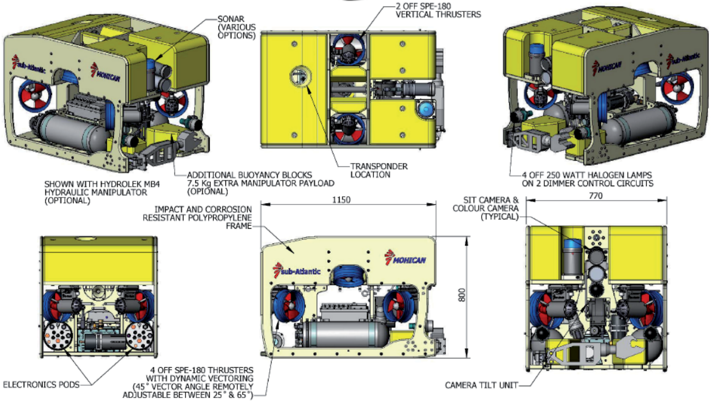
Mohican ROV Dimensions
