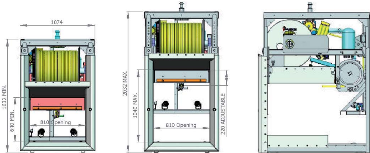
Size 1 TMS Dimensions
