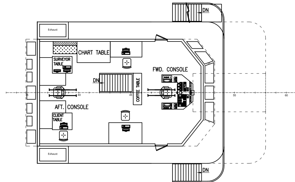
NAV. BRIDGE DECK PLAN
