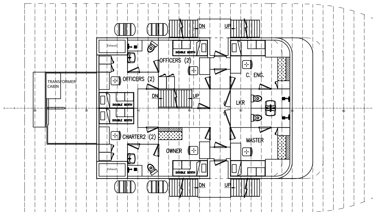
ACCOMMODATION DECK PLAN
