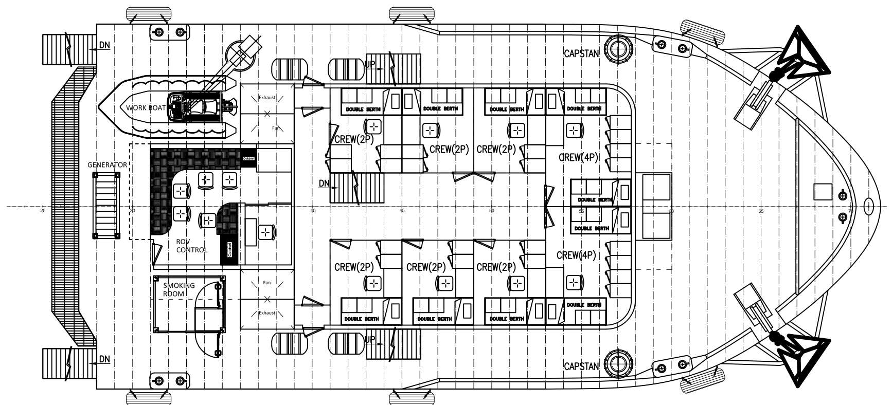
FORECASTLE DECK PLAN
